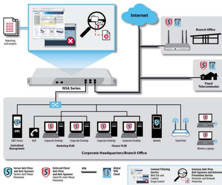
Figure 3. SonicWALL's NSA Series combines powerful Application Firewall controls with high-speed intrusion prevention, file and content inspection, and an extensive array of advanced networking and flexible configuration features.
